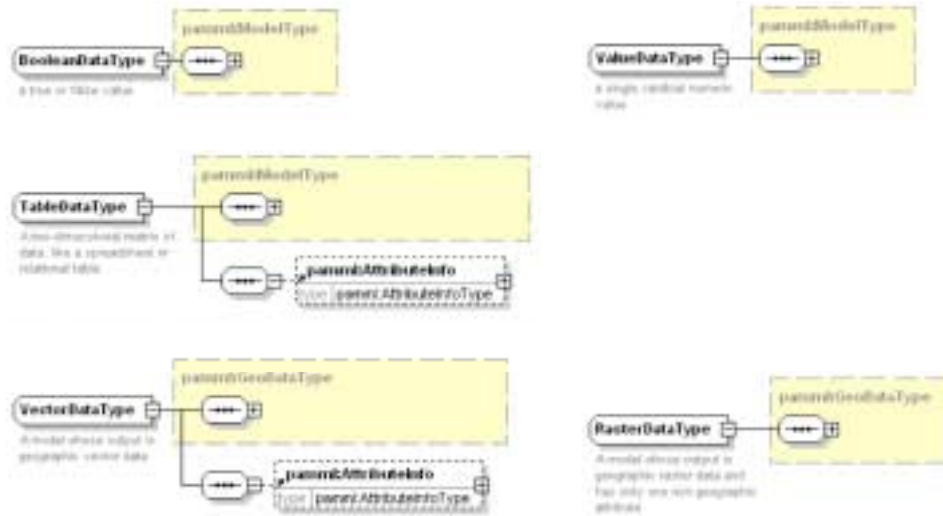
Figure 5-5: Some basic data models
