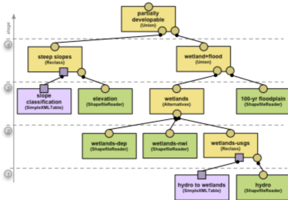
Figure 6-5: PAMML model of lands with development constraints
