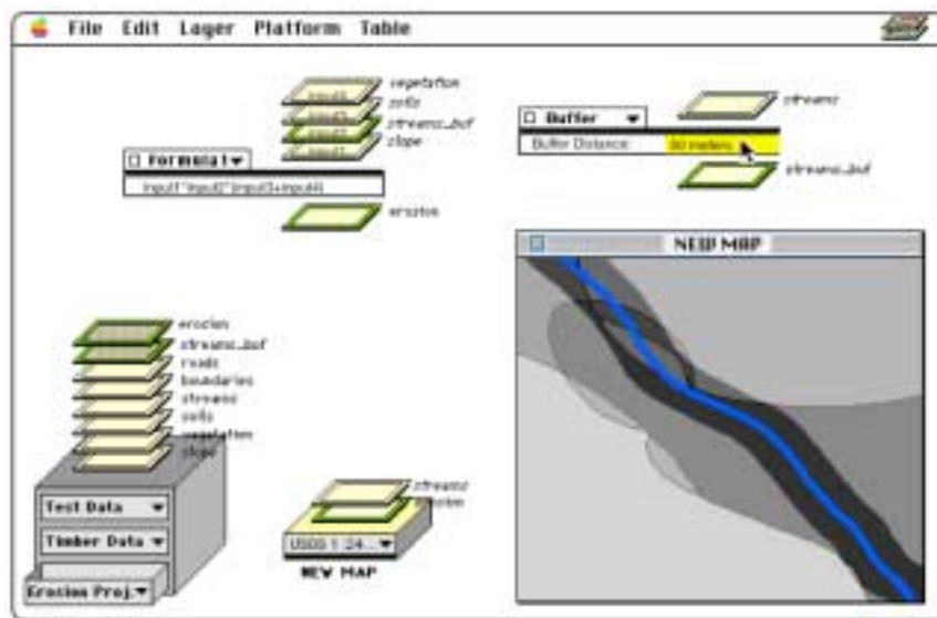
Figure 6-10: Visual Map Algebra as used in the Geographer's Toolkit
