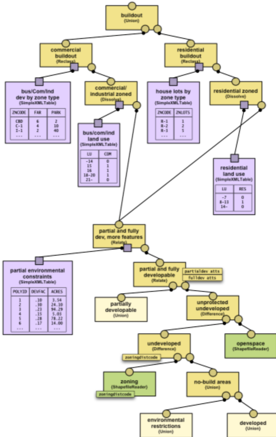
Figure 6-7: PAMML model of buildout (“partially developable”, “environmental restrictions”, and “developed” models are summaries of models shown above)
