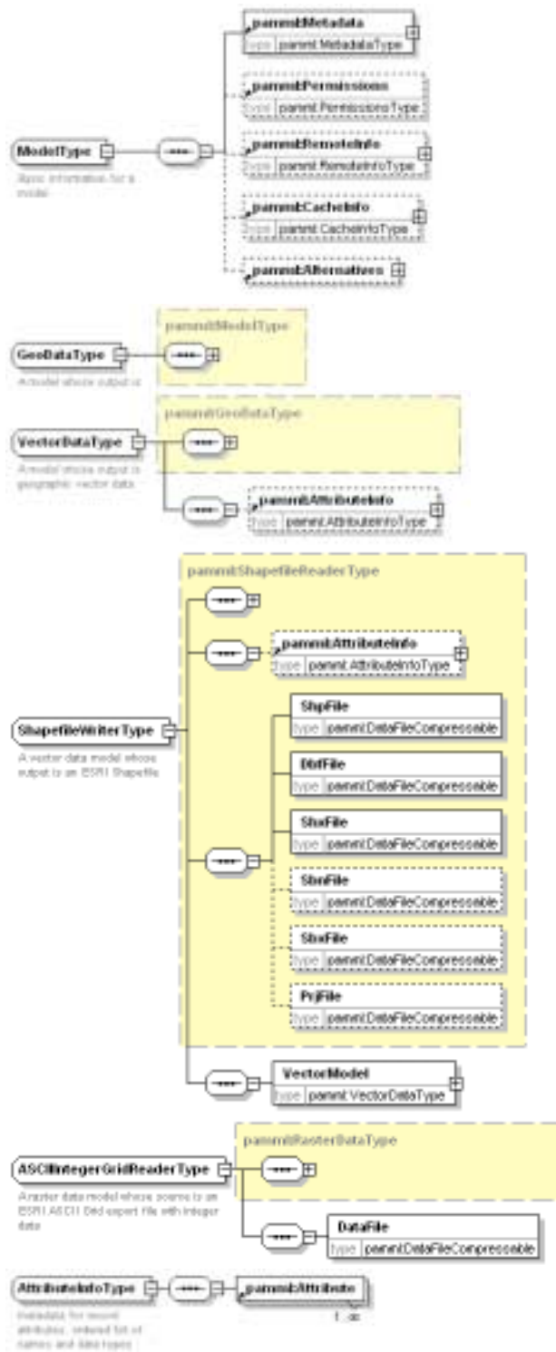
Figure 4-1: Common spatial data objects
