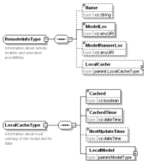
Figure 4-2: RemoteInfoType and LocalCacheType object diagrams
