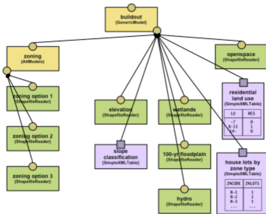
Figure 6-3: Buildout model showing alternative zoning options
