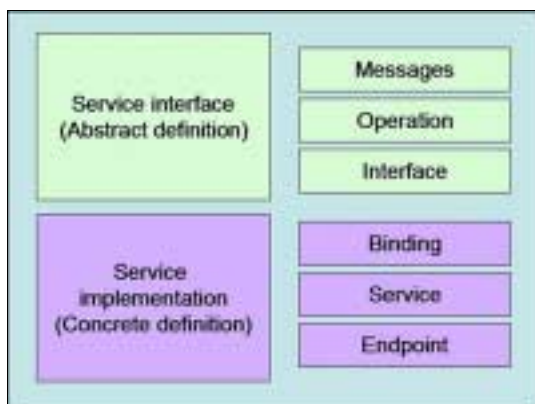
Figure 2-3: WSDL conceptual model
