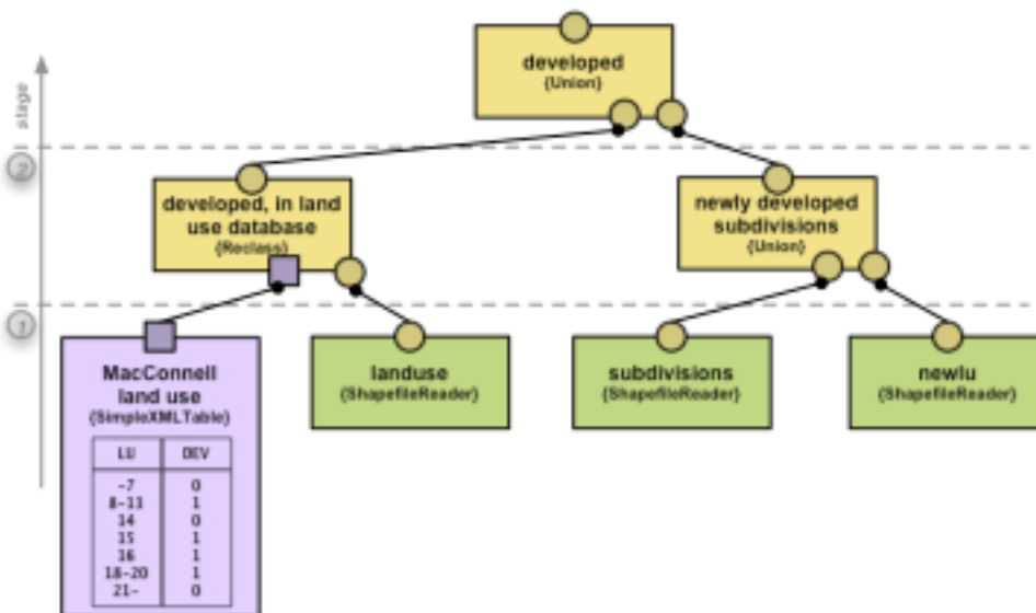
Figure 6-4: PAMML model of developed land
